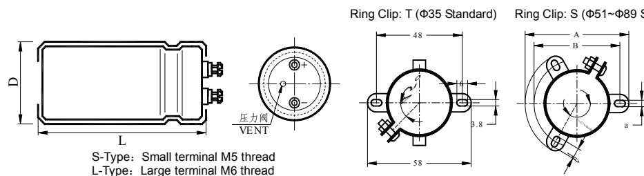
Ring Clip: T (Φ35 Standard)
